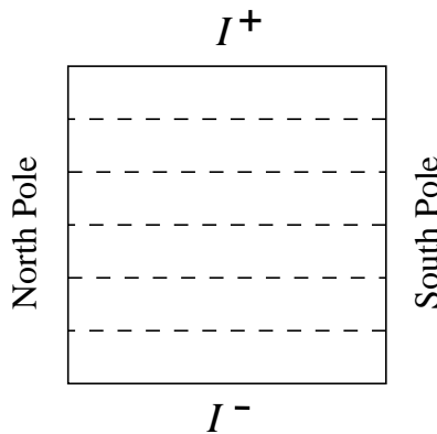
Fig. 2: Lines of constant \tau in global spherical coordinates are the spacelike two-spheres indicated by dashed lines.
