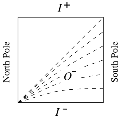
Fig. 1: Penrose diagram for dS_3 . Every point in the interior of the diagram is an S^1 . A horizontal line is an S^2 , with the left (right) vertical boundary being the north (south) pole. O^- is the region below the diagonal, and comprises the causal past of an observer at the south pole. The dashed lines are non-compact surfaces of constant t .
