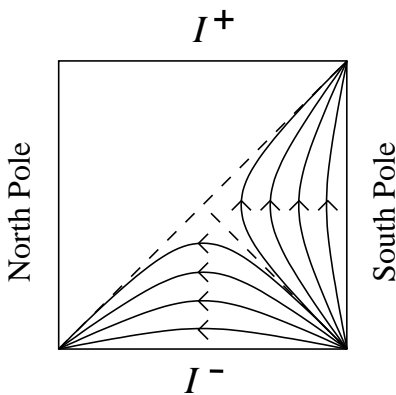
Fig. 3: The arrows indicate the direction of the Killing flow generated by L_0 + \bar{L}_0 within \mathcal{O}^- . Note that it is timelike along the worldline of an observer at the south pole but becomes spacelike on \hat{\mathcal{I}}^- .
