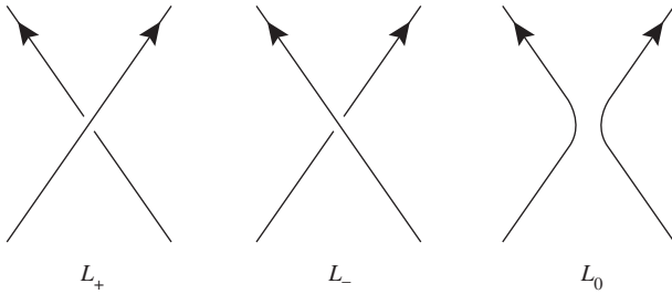
Fig. 12. Three skein-related links, L_+ , L_- and L_0 .
