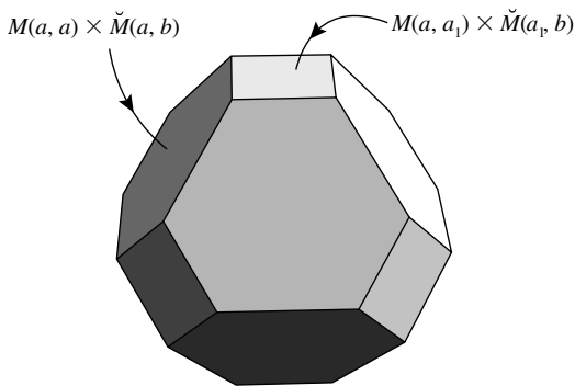
Fig. 6. A picture of the combinatorics of M^+(a, b) in the case that \bar{M}(a, b) is a 3-torus carrying a standard Morse function. Two of the codimension-1 faces are labelled. The critical point a_1 has index 1 less than a .
