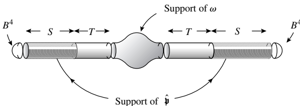
Fig. 10. The manifold X(S, T) obtained by adding cylinders and two 4-balls to W .
