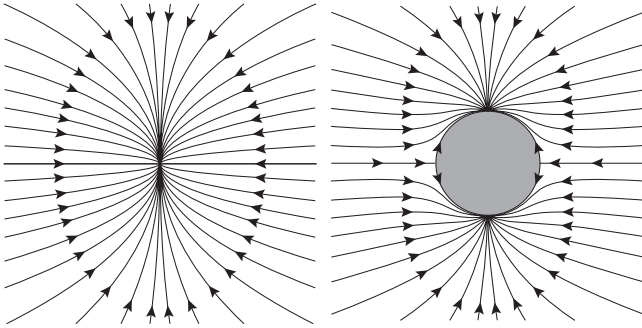
Fig. 2. A linear flow on \mathbb{R}^2 and the corresponding flow on the blow-up, S^1 \times \mathbb{R}^{\geq} .
