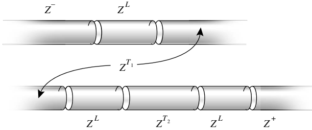
Fig. 5. Obtaining two doubly infinite cylinders by gluing the components of Z_T .
