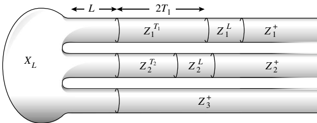
Fig. 7. Decomposing the cylindrical-end manifold X^* into the pieces (24.31).
