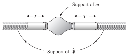
Fig. 9. Supports of \omega and \hat{\phi} separated by cylinders of length T in W(T) .
