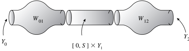
Fig. 8. The composite cobordism W(S) .
