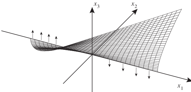
Fig. 4. Half of Whitney’s umbrella.
