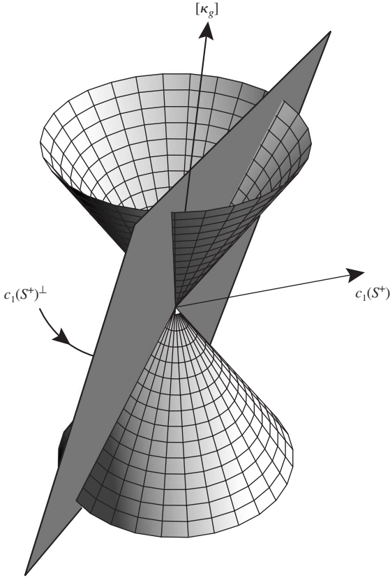
Fig. 11. Wall crossing when b^- \geq 10 and c_1(S^+) has negative square.
