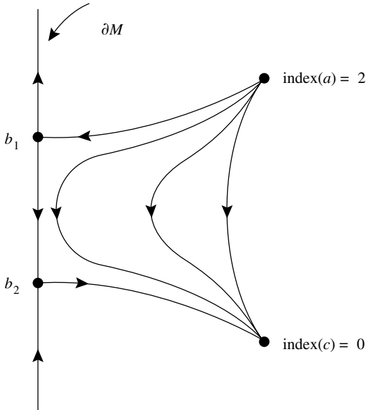
Fig. 1. A family of index-2 trajectories limiting to a 3-component broken trajectory.
