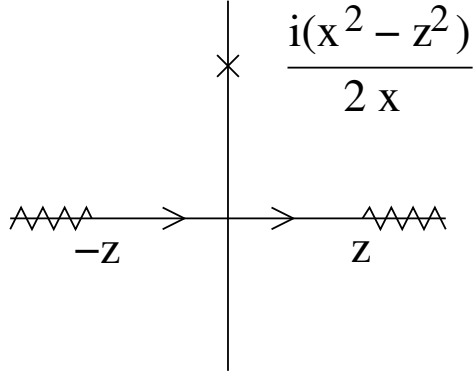
Figure 1: Integration contour for I_n . At large spacelike separation the pole is far up the imaginary axis. The pole moves down and crosses the integration contour when x = z ; one can continue to smaller values of x by deforming the contour. The integral may be singular when x \rightarrow 0^+ and the pole moves to -i\infty . There are singularities when x \rightarrow \pm iz and the pole hits an endpoint of the integration contour.
